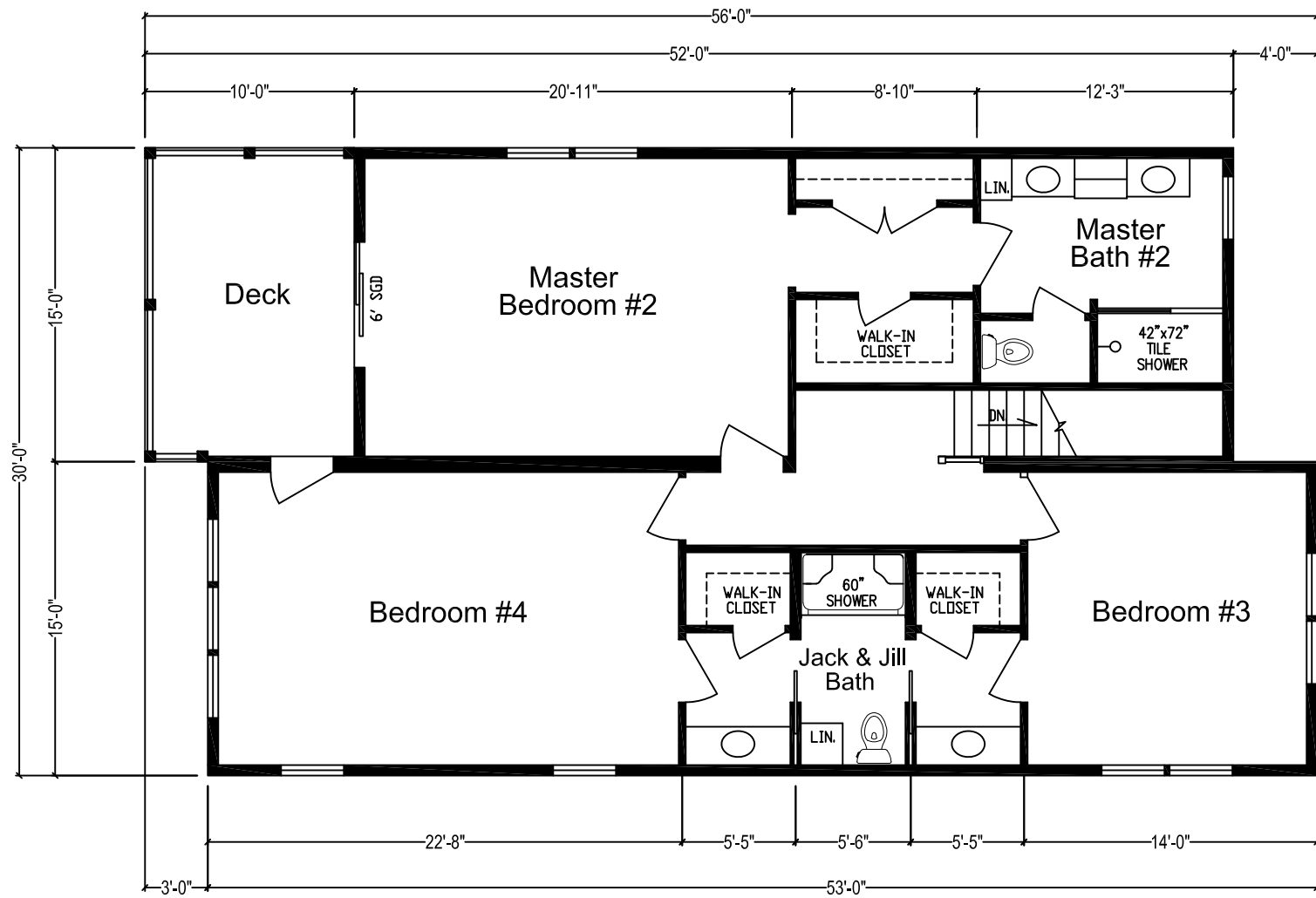
SECOND FLOOR
