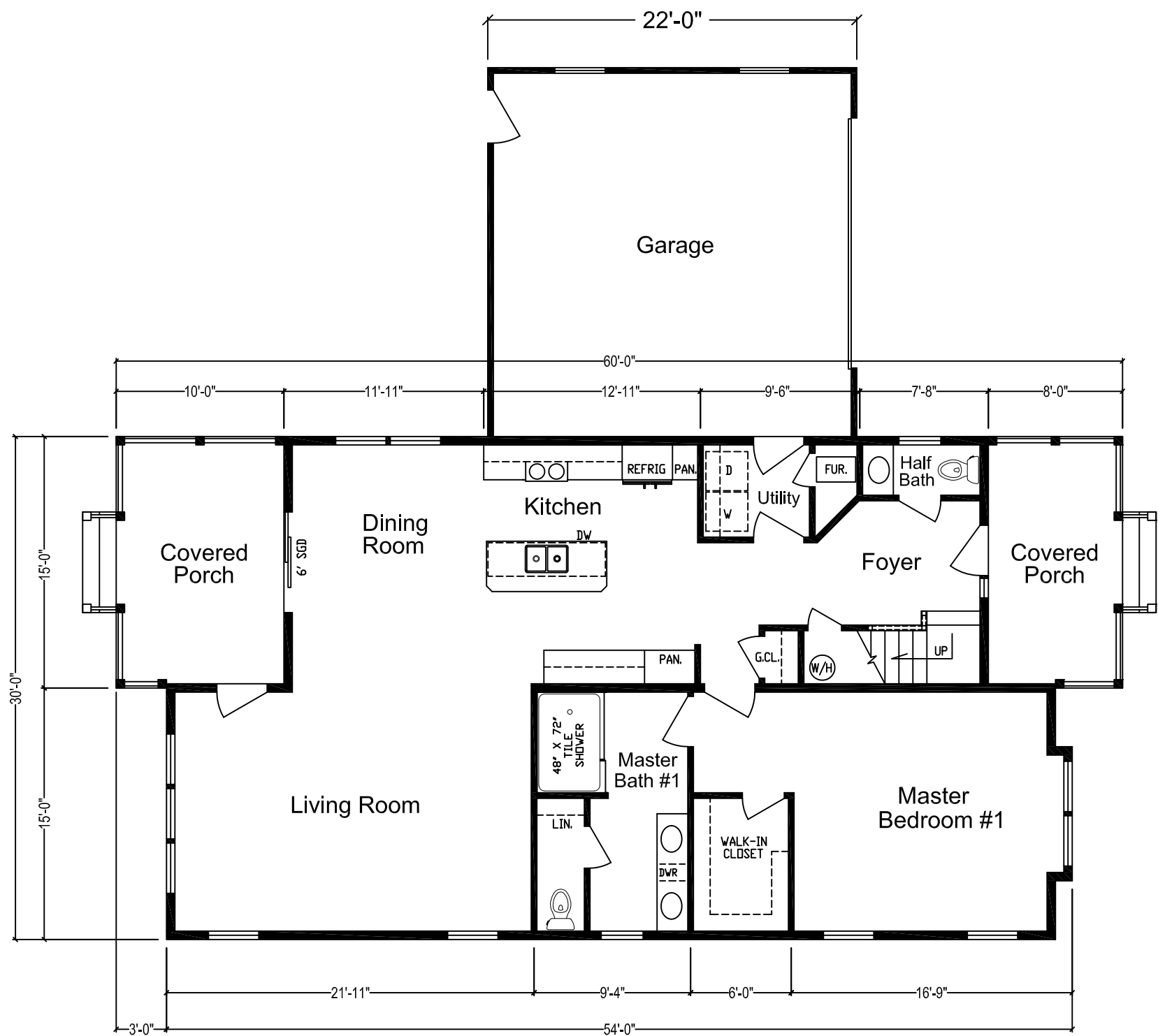
FIRST FLOOR
